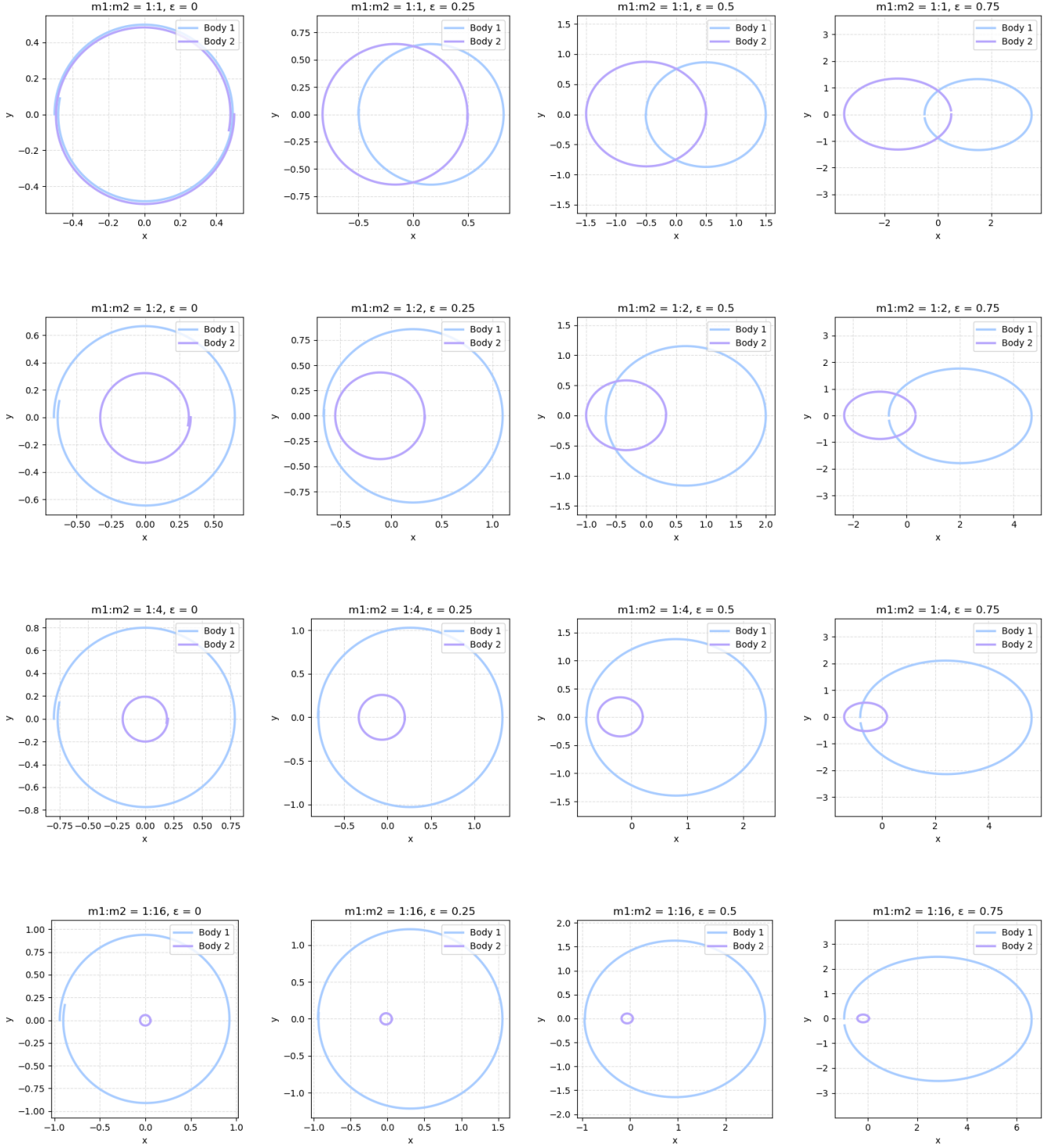
Figure 1. Two-body orbit plots for various mass ratios ( m_1 : m_2 from top to bottom) and eccentricities ( \epsilon from left to right).
